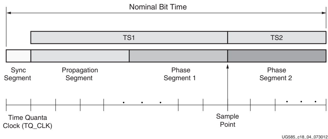
Figure 18-6: CAN Bit Time
