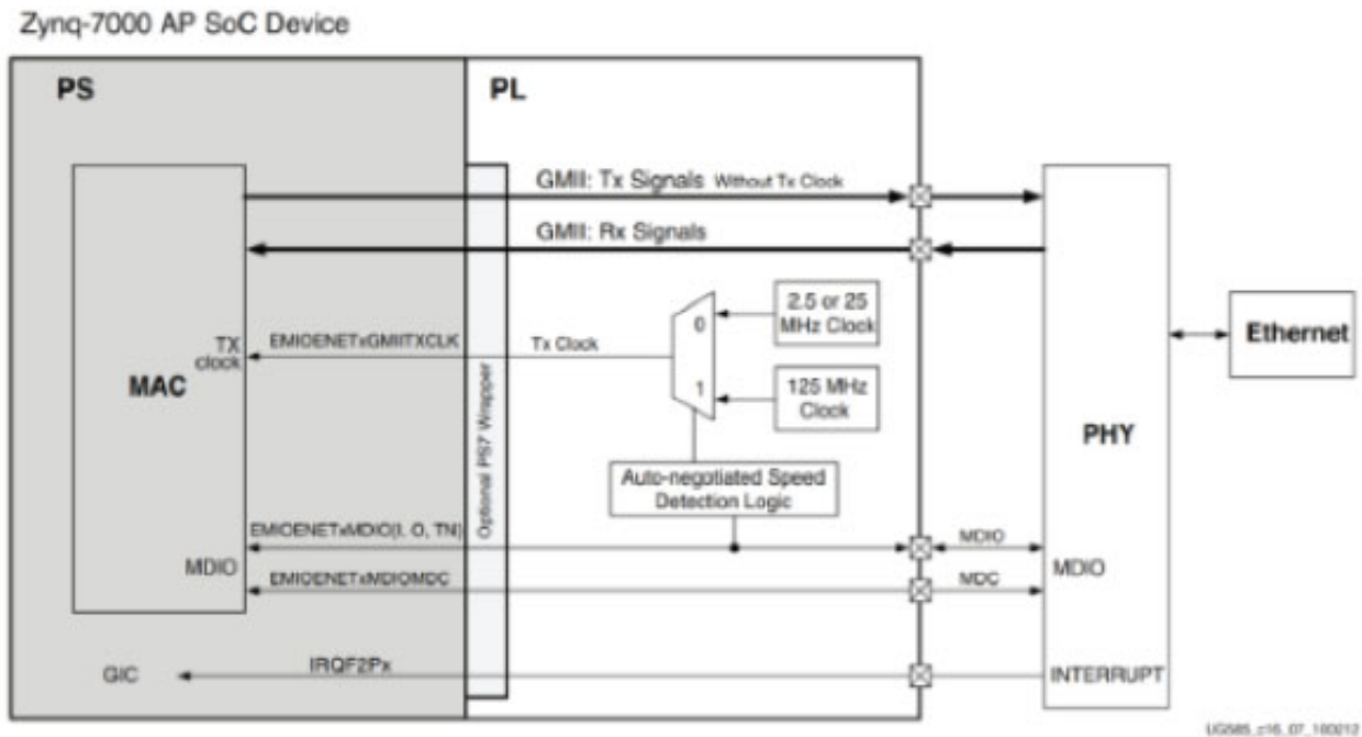
Figure 16-7: GMII Interface via EMIO Connections
