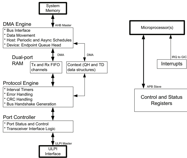
Figure 15-6: USB Controller Flow Diagram
