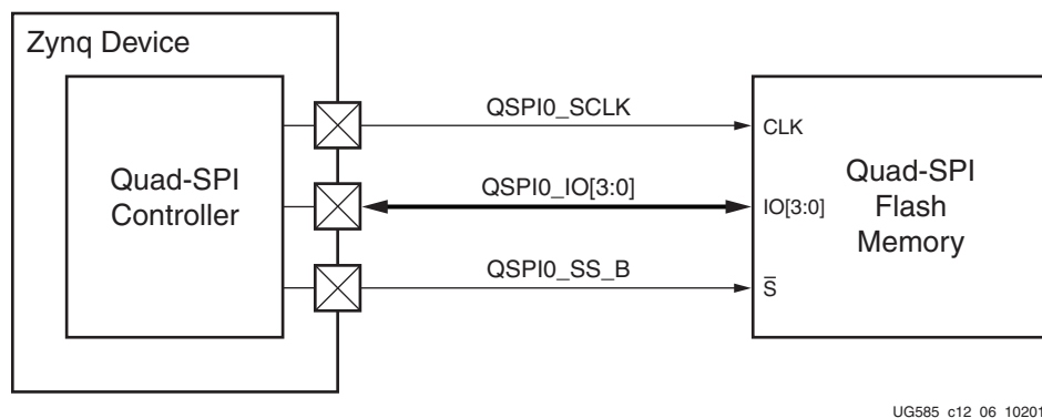
Figure 12-5: Quad-SPI Single SS 4-bit I/O
