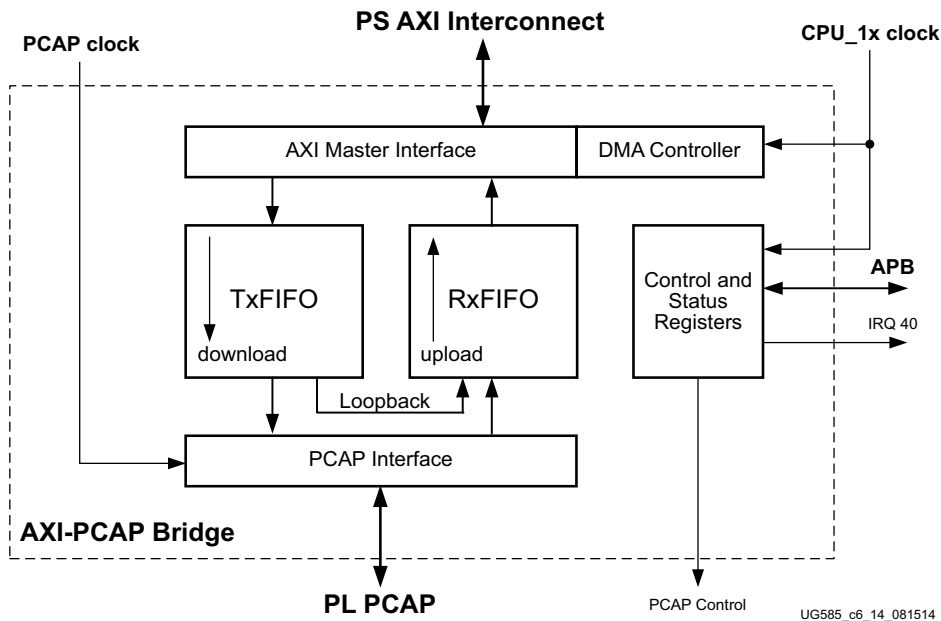
Figure 6-16: PCAP Bridge Architecture
