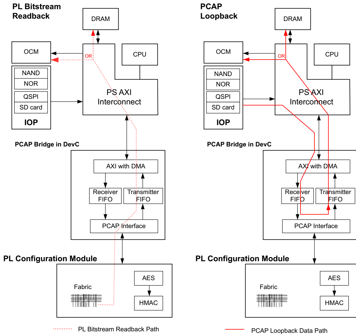
Figure 6-18: PL Bitstream Readback and PCAP Loopback Diagrams
