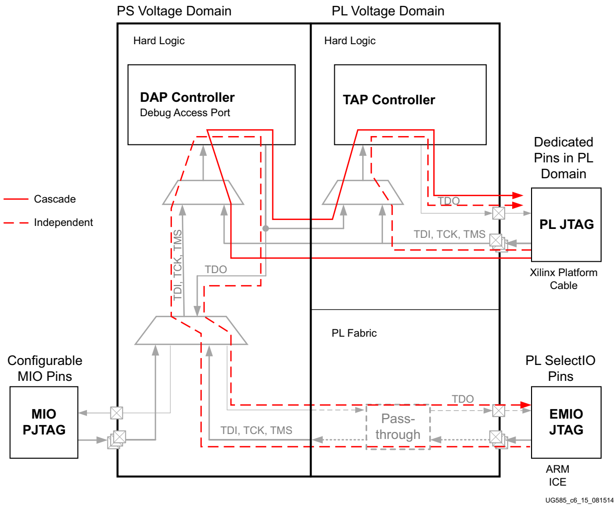
Figure 6-6: PS Cascade and Independent JTAG Chain Diagram
