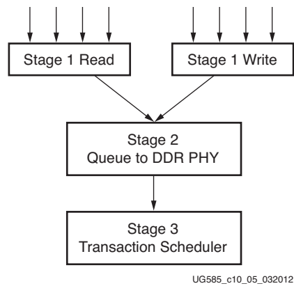
Figure 10-5: DDRC Arbitration
