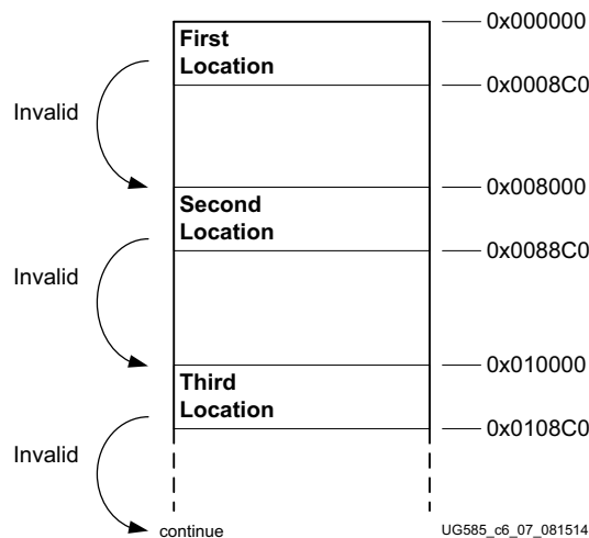
Figure 6-7: BootROM Header Search
