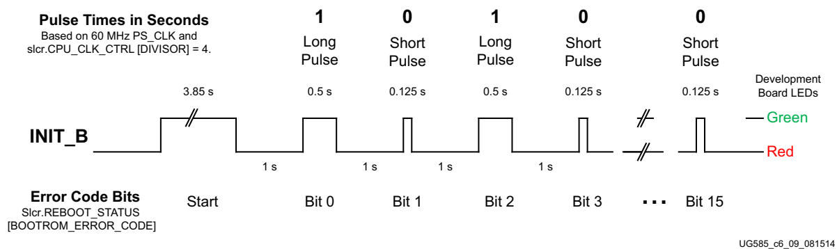
Figure 6-9: Error Code INIT_B Bit Waveform Example
