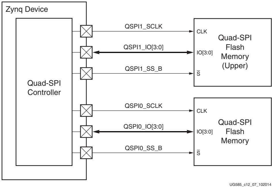
Figure 12-6: Quad-SPI Dual SS, 8-bit Parallel I/O
