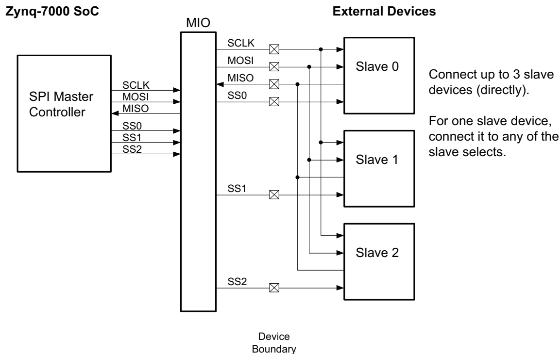
Figure 17-7: SPI Master Mode Wiring Diagram via MIO
