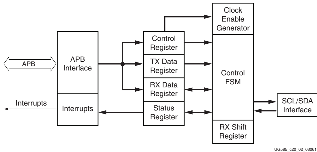
Figure 20-2: I2C Peripheral Block Diagram
