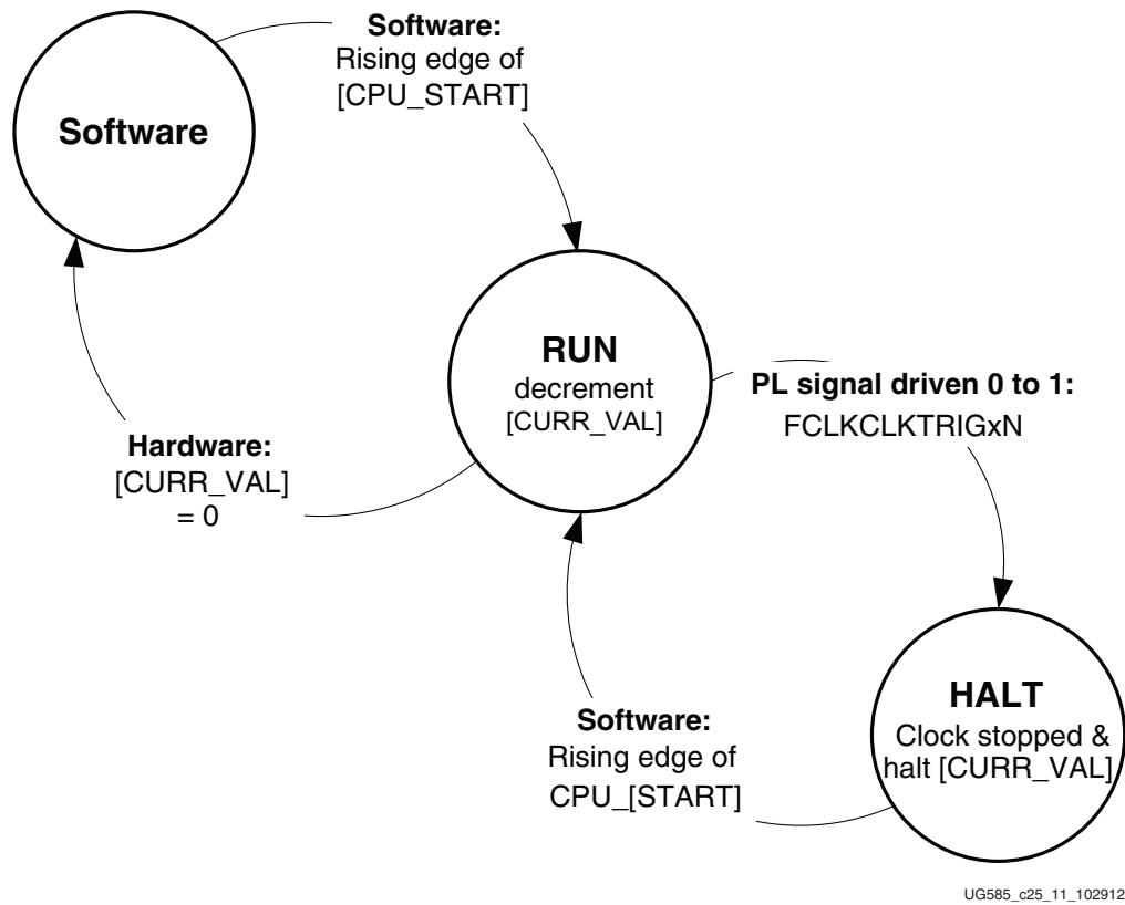
Figure 25-11: PL Clock Throttle States
