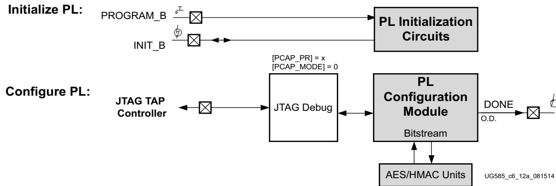
Figure 6-19: PL Initialization and Configuration Using User-JTAG
