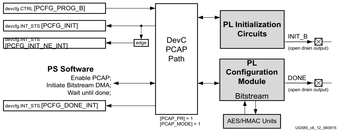
Figure 6-11: PCAP Path for PL Initialization and Configuration
