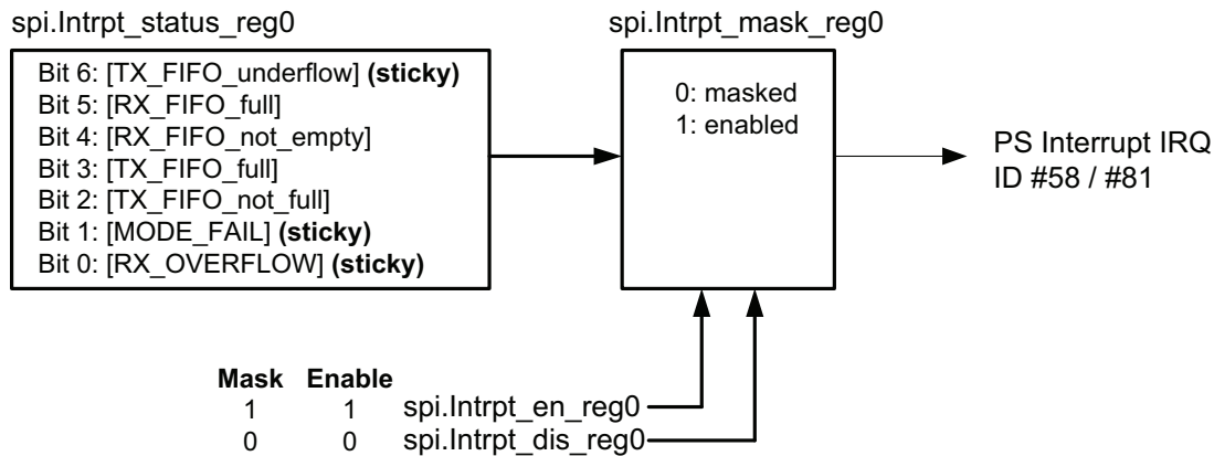
Figure 17-4: SPI Interrupt Register Bits, Logic Flow
