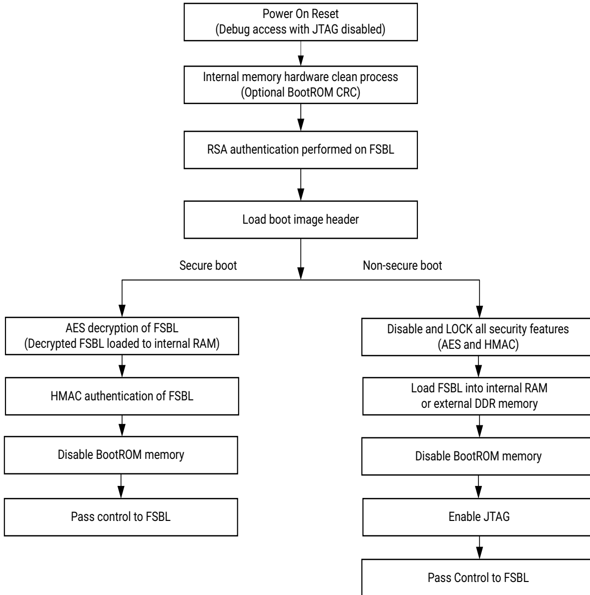
Figure 32-2: PS Boot Flow
