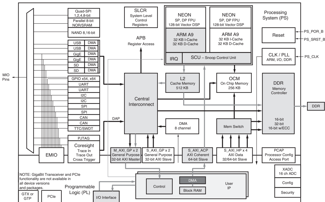
Figure 22-4: Example ACP DMA Topology
