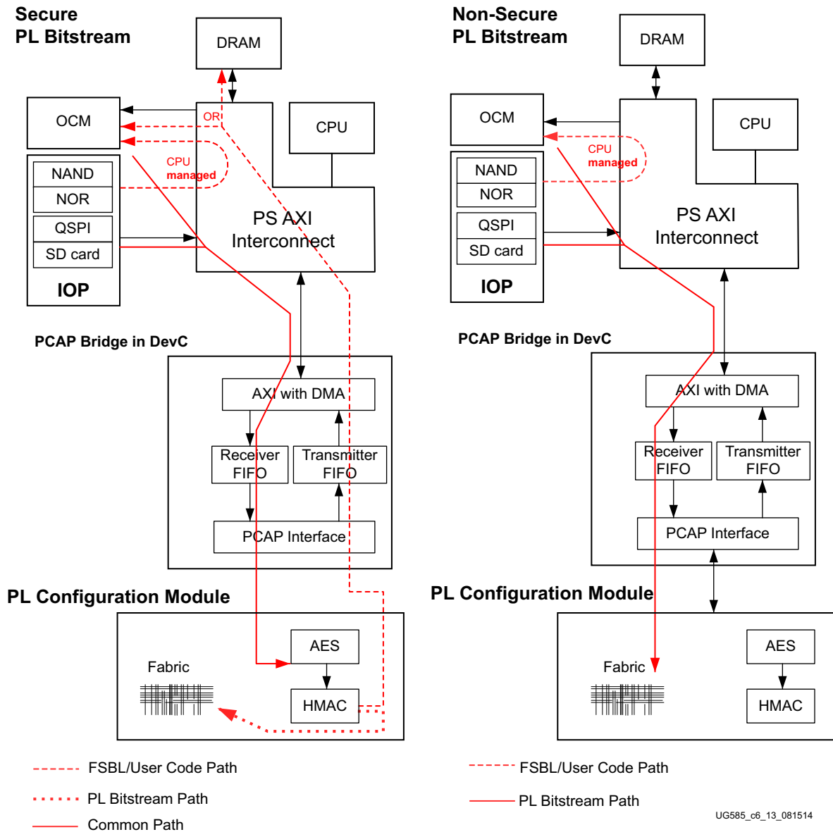
Figure 6-17: Non-Secure and Secure PL Bitstream Path Diagrams
