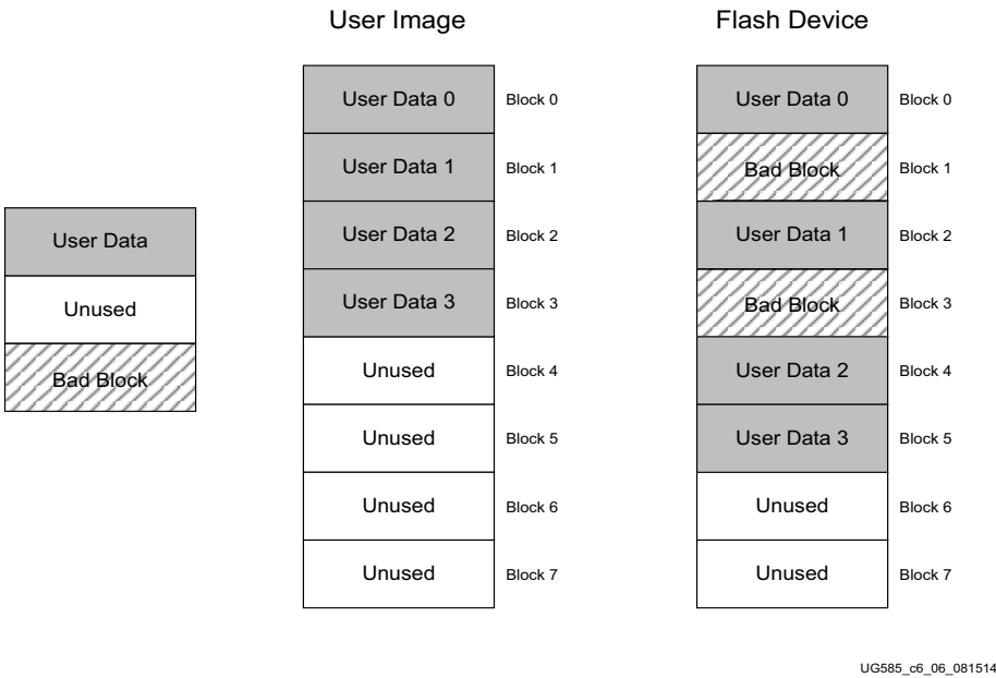
Figure 6-5: NAND Flash Device with Bad Blocks Example
