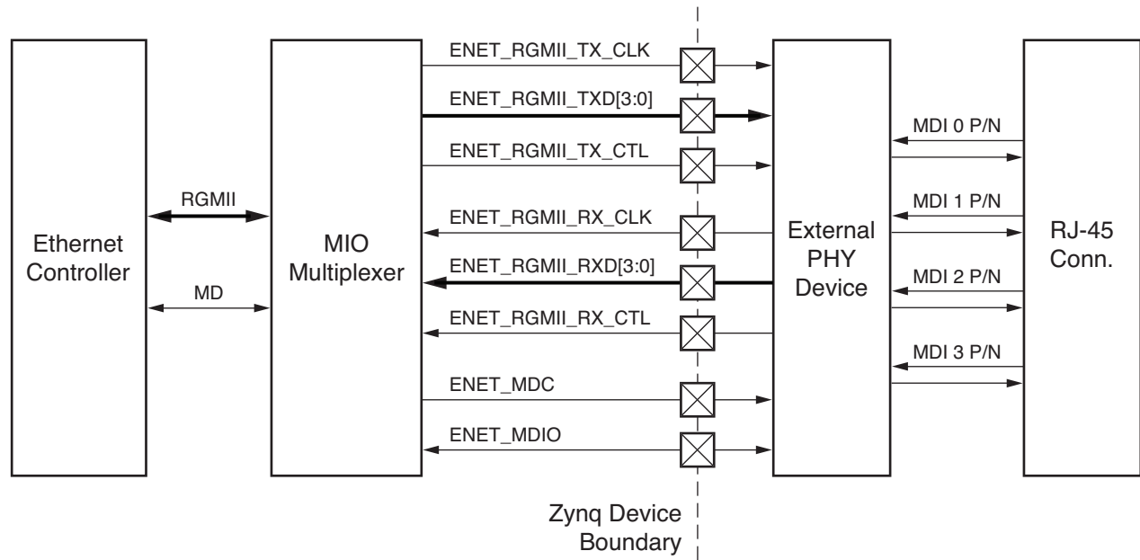
Figure 16-6: Ethernet Communications Wiring Connections
