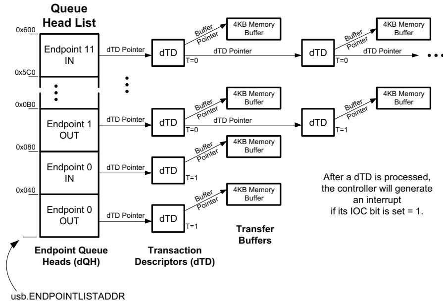
Figure 15-13: USB Device Link-list Endpoints Example
