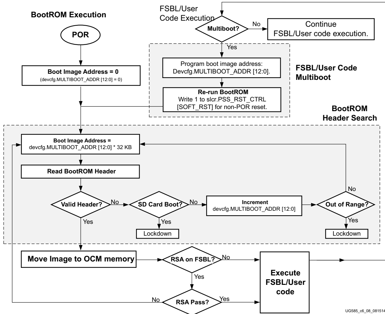
Figure 6-8: BootROM Header Search and FSBL/User Code Multiboot Flowchart
