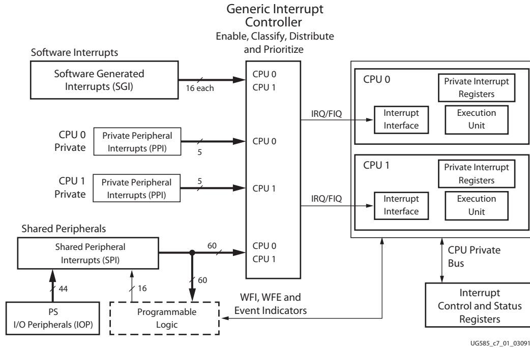
Figure 7-1: System-Level Block Diagram
