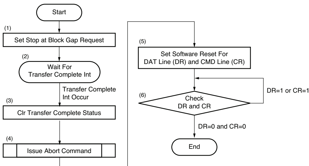
Figure 13-6: SDIO Controller Synchronous Abort Sequence
