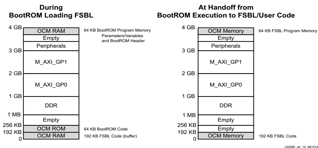
Figure 6-10: System Memory Map During BootROM Execution
