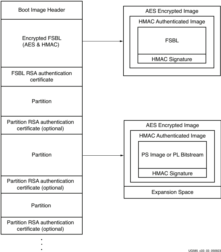
Figure 32-3: Secure Boot Image Format
