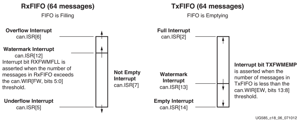
Figure 18-4: CAN RxFIFO and TxFIFO Watermark Interrupts
