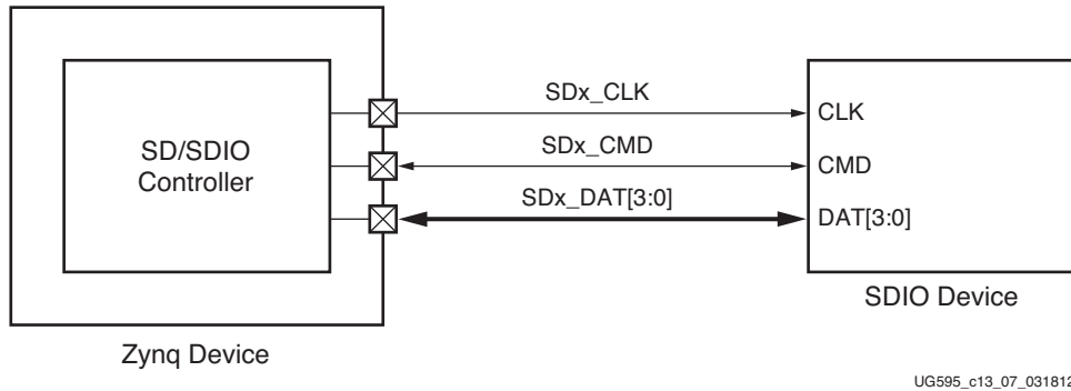
Figure 13-7: SDIO Controller Device Wiring Diagram
