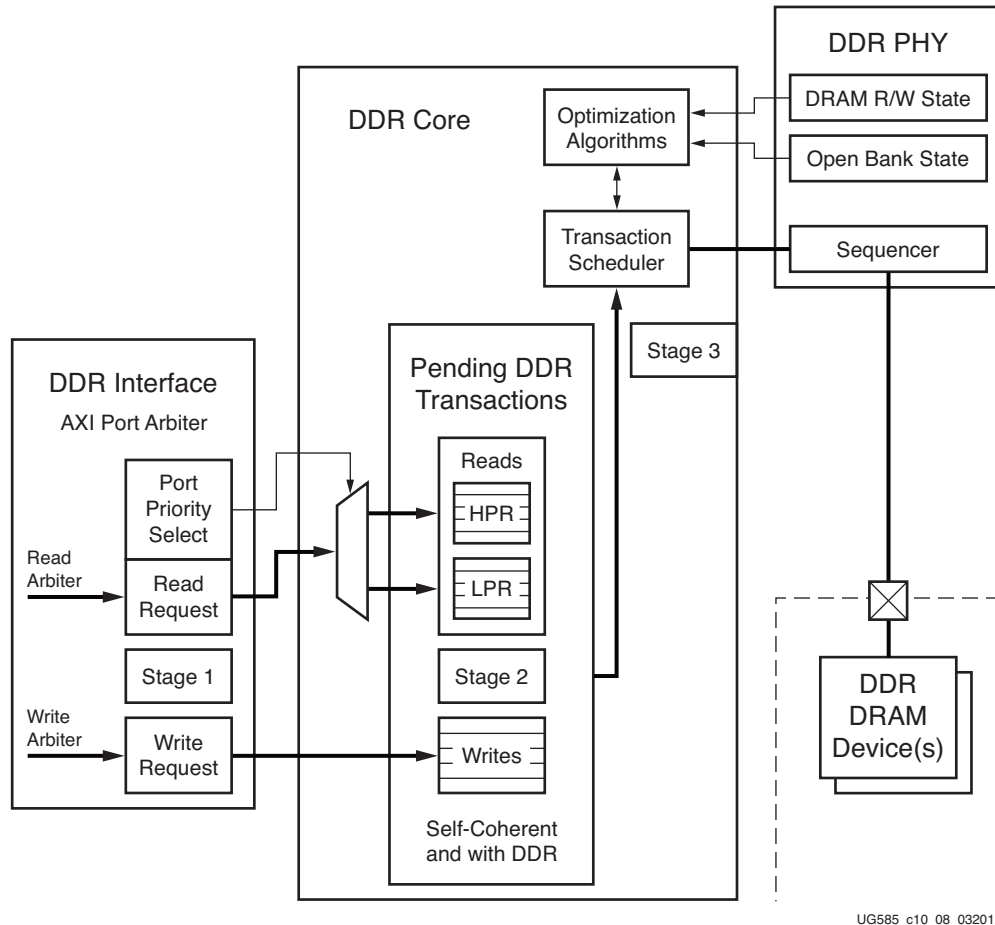
Figure 10-8: Read Queue
