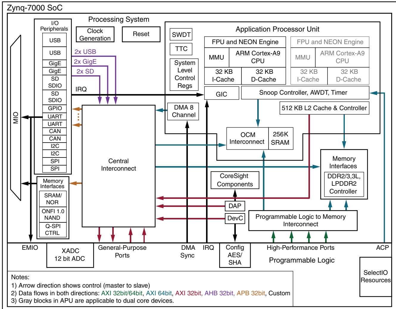
Figure 1-1: Zynq 7000 SoC Overview
