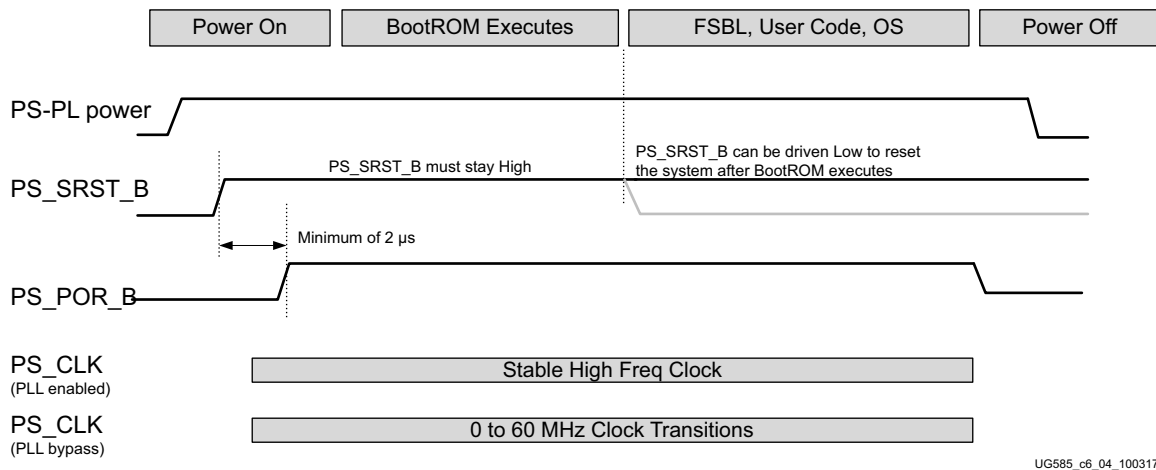
Figure 6-4: Power and Reset Sequencing Waveform
