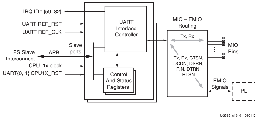
Figure 19-1: UART System Viewpoint
