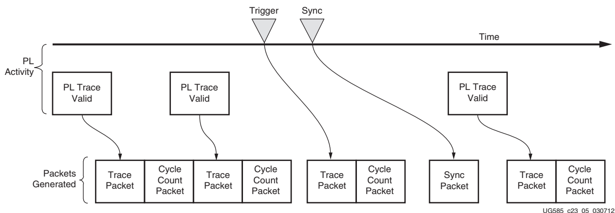
Figure 23-5: Packet Generation, Synchronization Case
