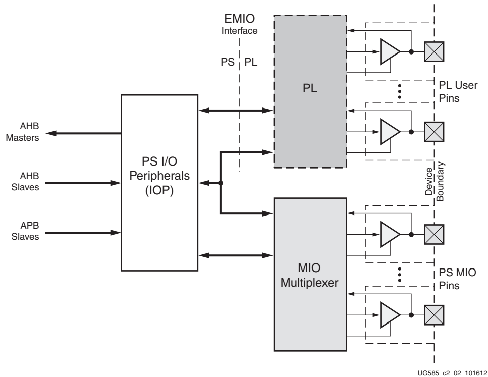
Figure 2-2: MIO-EMIO Overview
